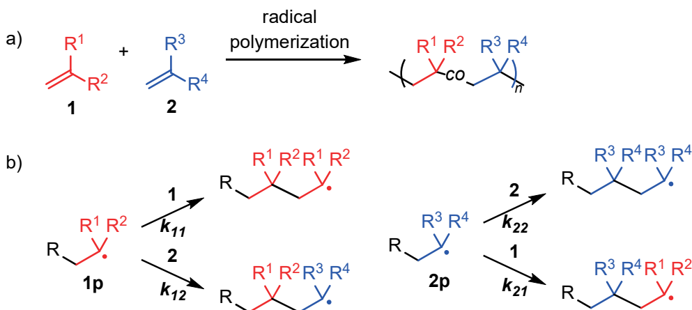
Fig. 1. Copolymerization: (a) the general reaction scheme and (b) the four propagation pathways involving the copolymerization.
