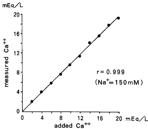
Fig. 19. Standard curve of Ca ++ for calibration. The regression coefficient was 0.999 in the range of 2 to 20 mEq/L.
