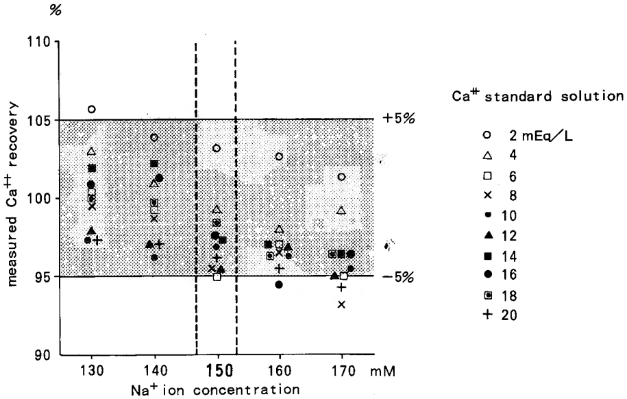
Fig. 20. Effects of \text{Na}^{+} ion on measured \text{Ca}^{++} .
