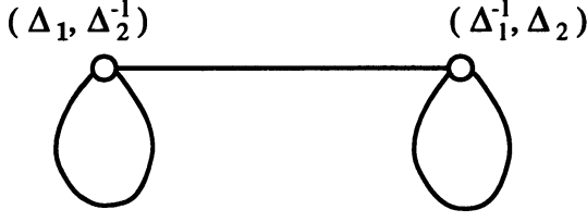
Figure 1: The price transition graph G of the class The return of portfolios
