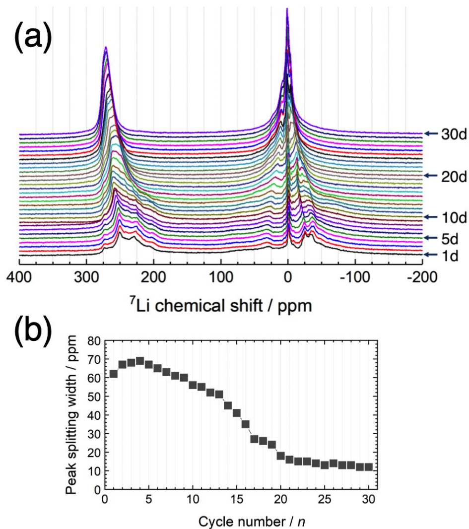
Fig. 3. (a) Operando ^7\text{Li} NMR spectra of the FeF 3 electrode at the fully charged states during 30 cycles. The cell was cycled at a current density of 71.2 \text{ mA g}^{-1} . (b) Evolution of the splitting width between the peaks at -35 and 30 ppm in the lowermost spectrum in (a).
