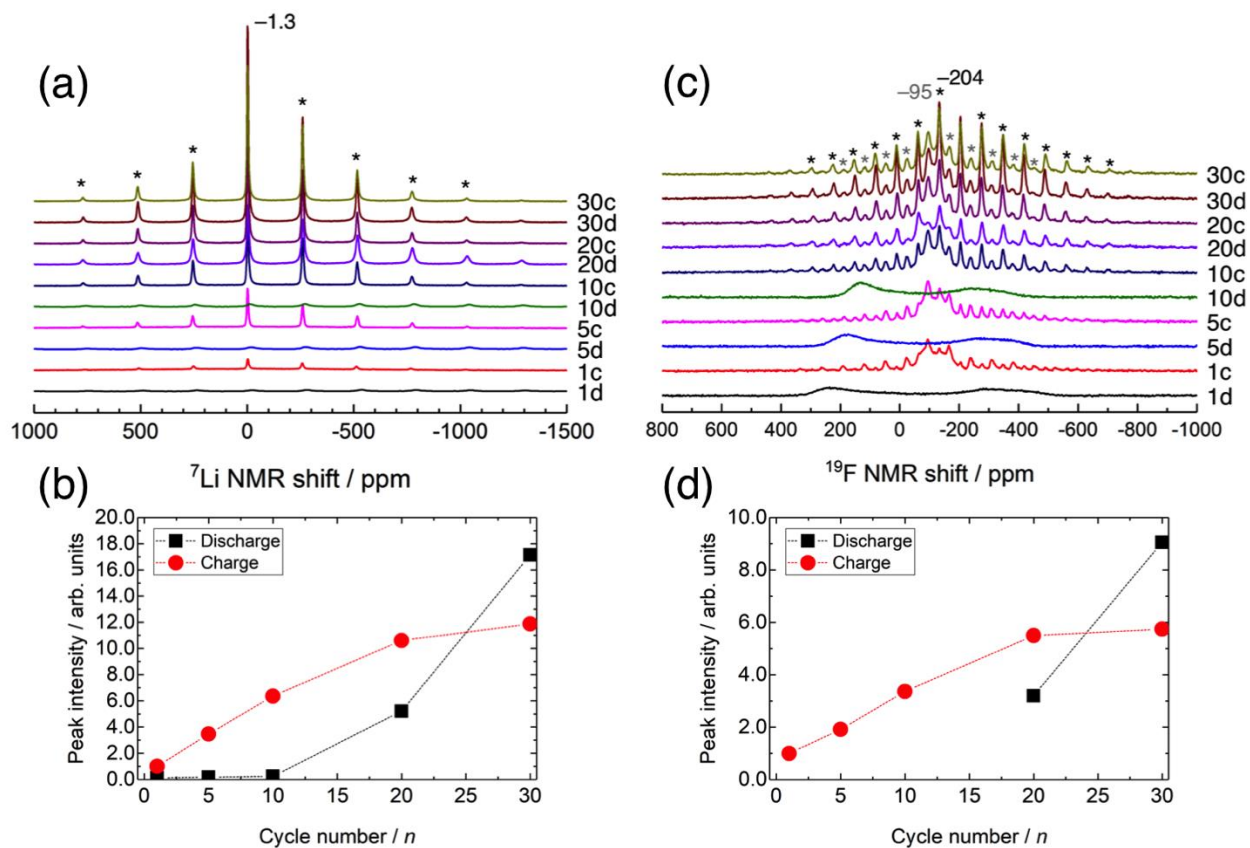
Fig. 4. (a) ^7\text{Li} MAS NMR spectra of the \text{FeF}_3 electrode during discharge–charge cycles and (b) normalized ^7\text{Li} intensity evolution of LiF signal at -1.3 ppm, and (c) ^{19}\text{F} MAS NMR spectra and (d) normalized ^{19}\text{F} intensity evolution of LiF signal at -204 ppm. Asterisks indicate SSBs.
