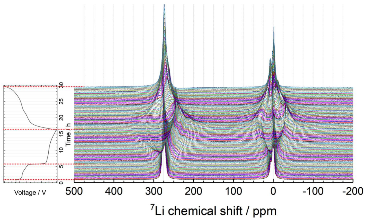
Fig. 2. Operando ^7\text{Li} NMR spectra of the \text{FeF}_3 electrode during the initial cycle. The cell was cycled between 1.0 and 4.5 V at a current density of 35.6 \text{ mA g}^{-1} .
