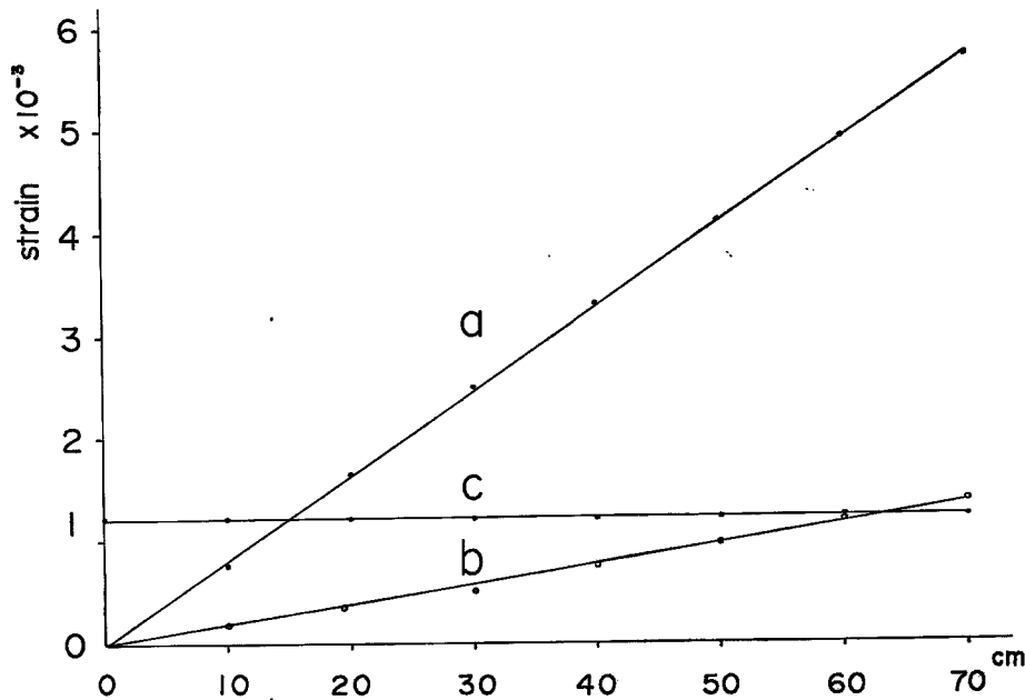
Fig. 4 The strain output relation between a guide pipe and a sensor when the guide pipe was bent from 0 to 70 cm.
