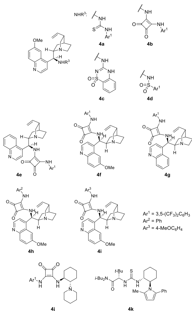
Fig. 1. Organocatalysts.
