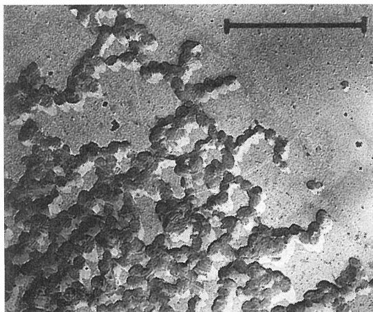
Fig. 4. Platelike polyethylene crystals developed in Experiment A.
