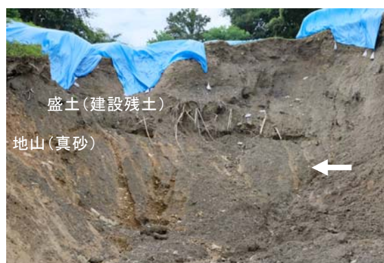
Photo 4 Internal structure of valley fill. White arrow shows the boundary between the fill material and the original ground
