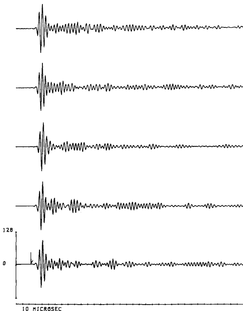
Fig. 5. Seismograms produced by model experiments for medium of Q=300 ( g=0.008 \text{ cm}^{-1} and Q_{\text{scat}}=520 ): the source origin time is marked with a vertical arrow.
