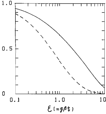
Fig. 1. Coda power ratios as a function of \varepsilon : solid curve, P_K/P_G ; dashed curve, P_{sin}/P_G ; \varepsilon , ratio of the distance traveled to the mean free path g^{-1} . P_{sin} , P_K and P_G denote coda power spectral densities by Aki and Chouet 2) , Kopnichev 13) and Gao et al 14) .
