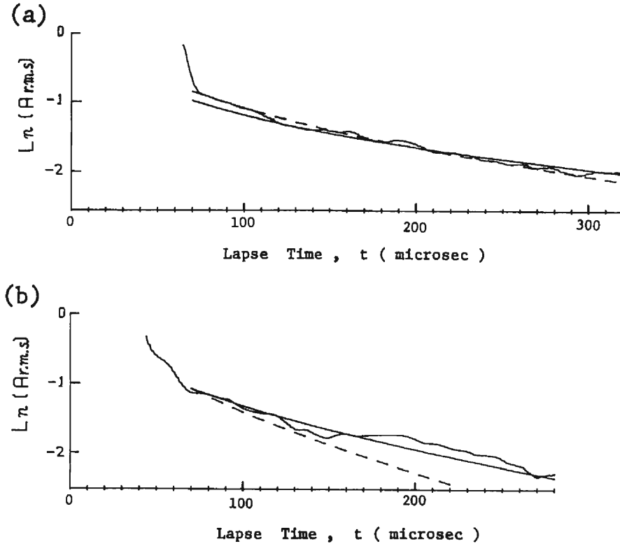
Fig. 7. Observed and predicted coda decays with time. (a) for medium with Q=300 ( g=0.008 \text{ cm}^{-1} and Q_{scat}=520 ); (b) for medium with Q=150 ( g=0.024 \text{ cm}^{-1} and Q_{scat}=220 ). Solid curves denote coda amplitude decays predicted by the multiple-scattering model of Gao et al. and dashed curves by the single-scattering model.
