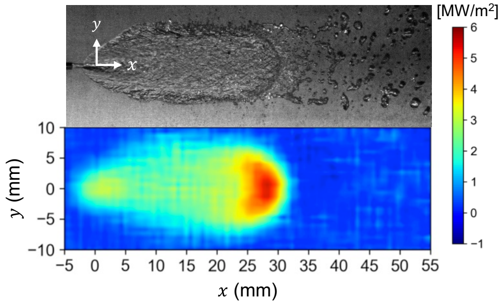
Fig. 16 Direct image of liquid film and distribution of heat flux at t = 0.6 s under the condition of d = 0.7 mm and \dot{m} = 5.0 g/s.
