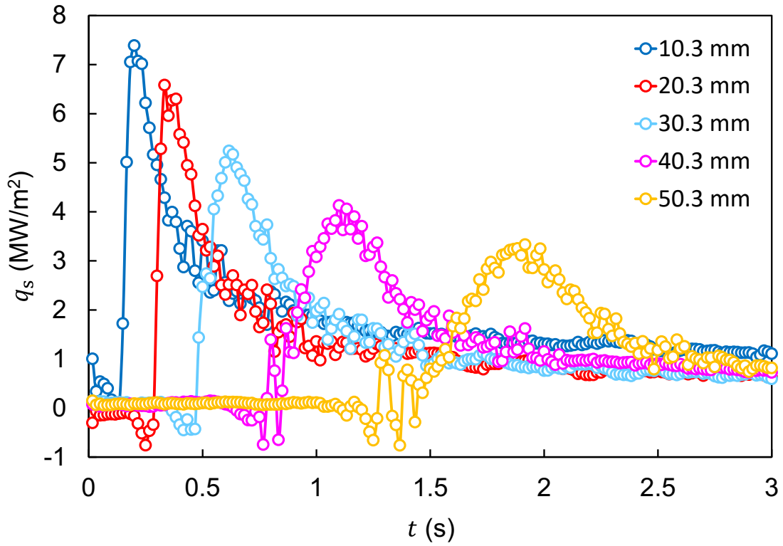
Fig. 13 Time history of heat flux at each position on the x -axis under the condition of d = 0.7 mm and \dot{m} = 5.0 g/s.
