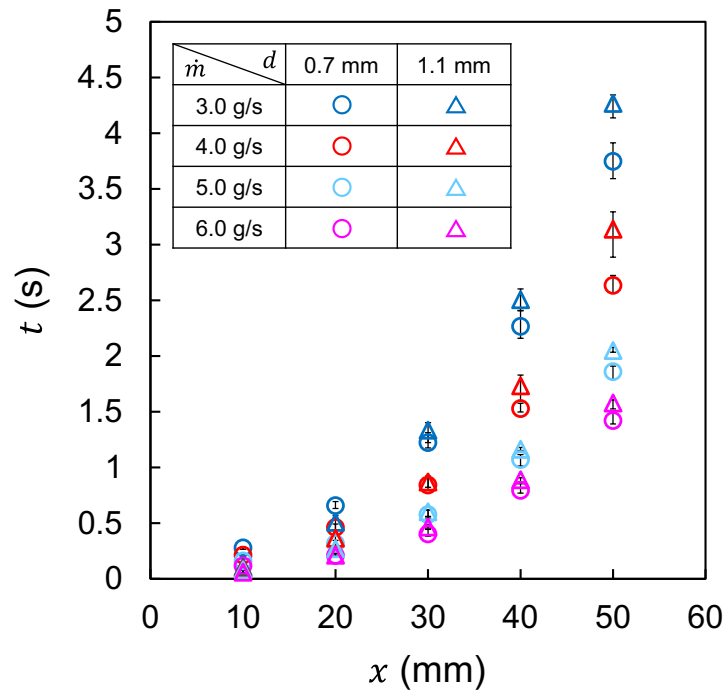
Fig. 8 Elapsed time when WF reaches certain positions on the x -axis.
