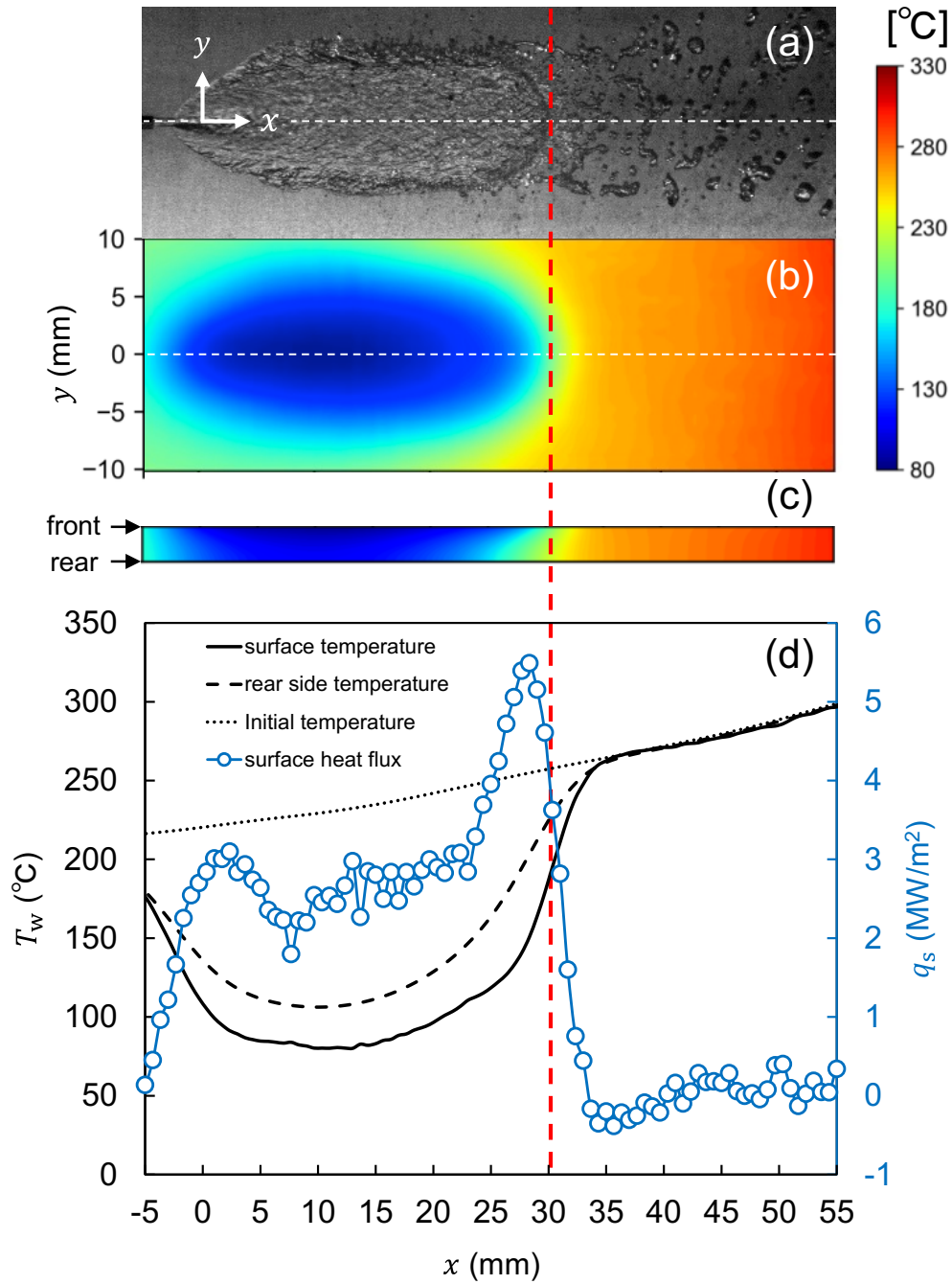
Fig. 6 Direct image of the liquid film (a), thermal images of temperature distribution of the front surface (b) and in the xz -plane for y = 0 (c), and estimated surface temperature and heat flux distribution along the x -axis for y = 0 calculated (d) at the elapsed time of 0.6 s. Red broken line indicates the WF position.
