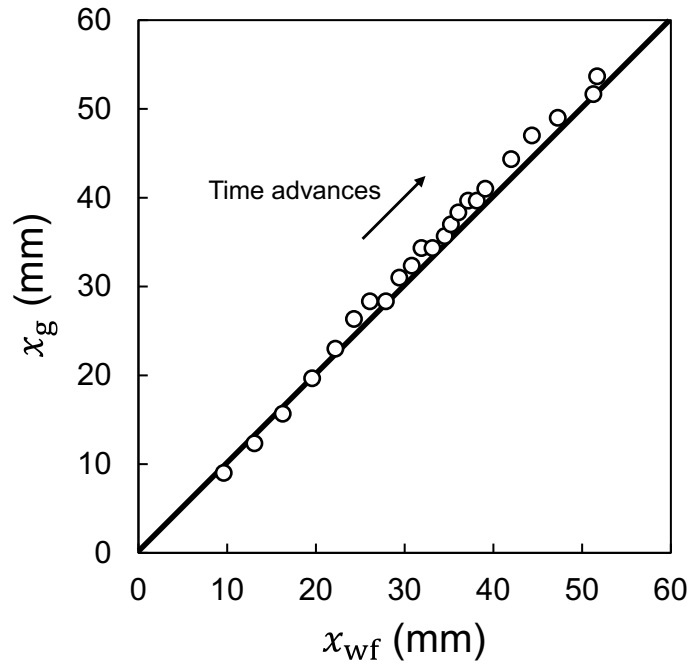
Fig. 7 Relationship between WF position and position where spatial temperature gradient takes its maximum value on the x -axis.
