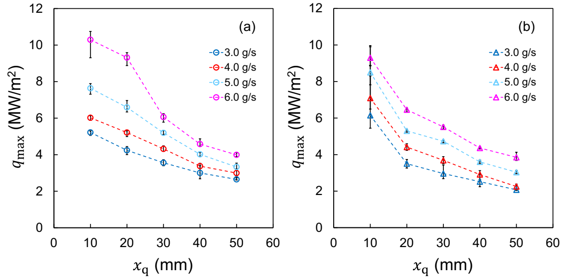
Fig. 15 History of maximum heat flux at each position on the x -axis under the condition of d = 0.7 mm (a) and d = 1.1 mm (b).
