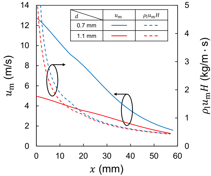
Fig. 9 Mean velocity of liquid film and film mass flow rate per unit liquid film width on the x axis under the condition of \dot{m} = 5.0 g/s predicted by the model in [24].
