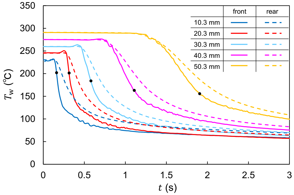
Fig. 11 Temperature history at each position on the x -axis under the condition of d = 0.7 mm and \dot{m} = 5.0 g/s. The black dots indicate the temperature at the moment when the WF reached each position.
