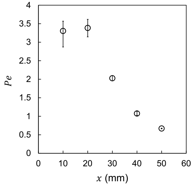
Fig. 12 Change in Peclet number under the condition of d = 0.7 mm and \dot{m} = 5.0 g/s.
