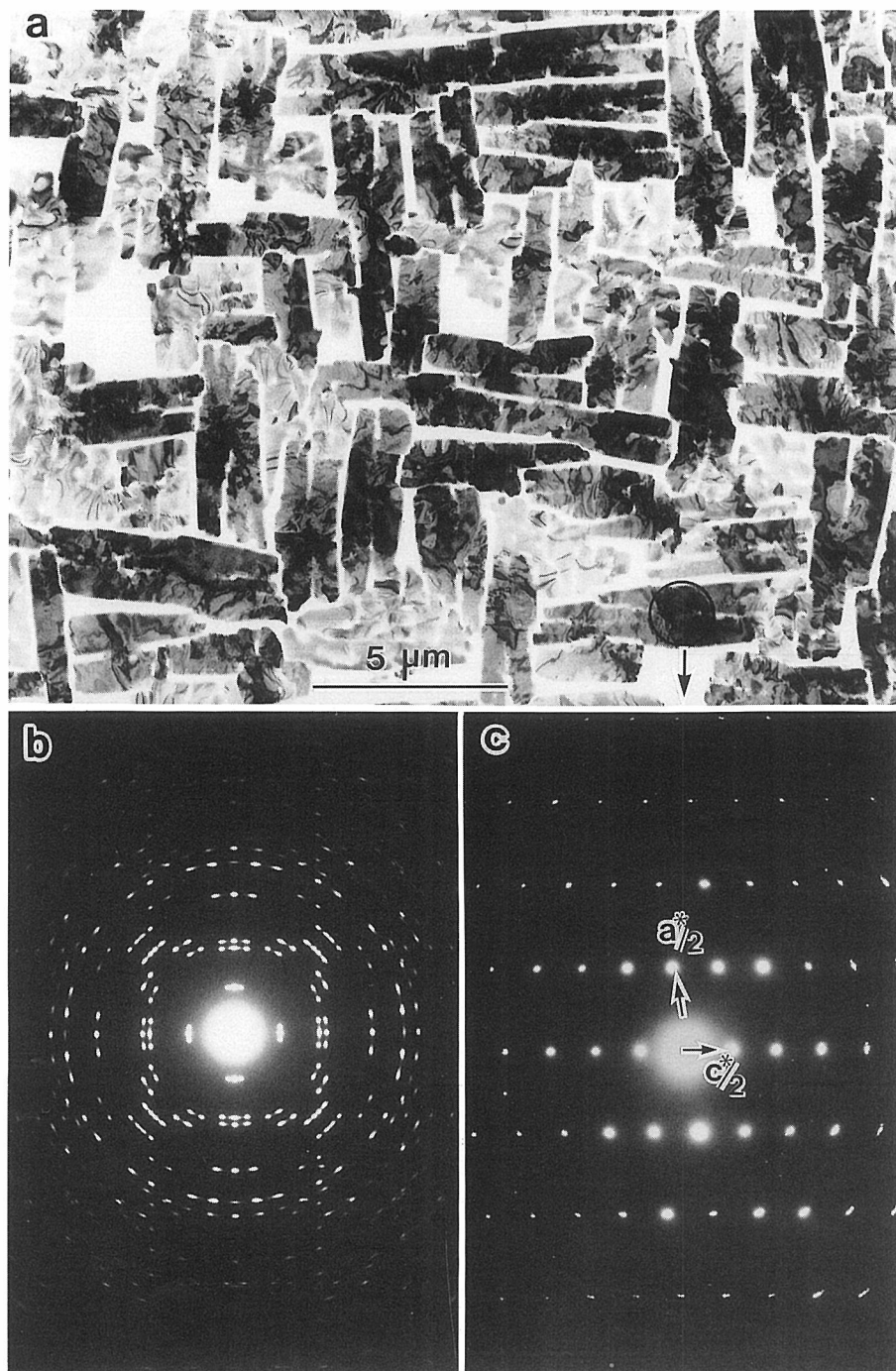
Fig. 2. Epitaxial film of TCNQ grown on KCl at 50°C (a) and high resolution electron diffraction pattern(b) from (a). A selected area electron diffraction pattern(c) was obtained from an encircled area in (a).
