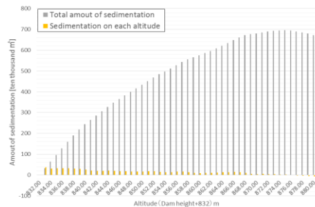
Fig. 8 Shape of reservoir sedimentation
