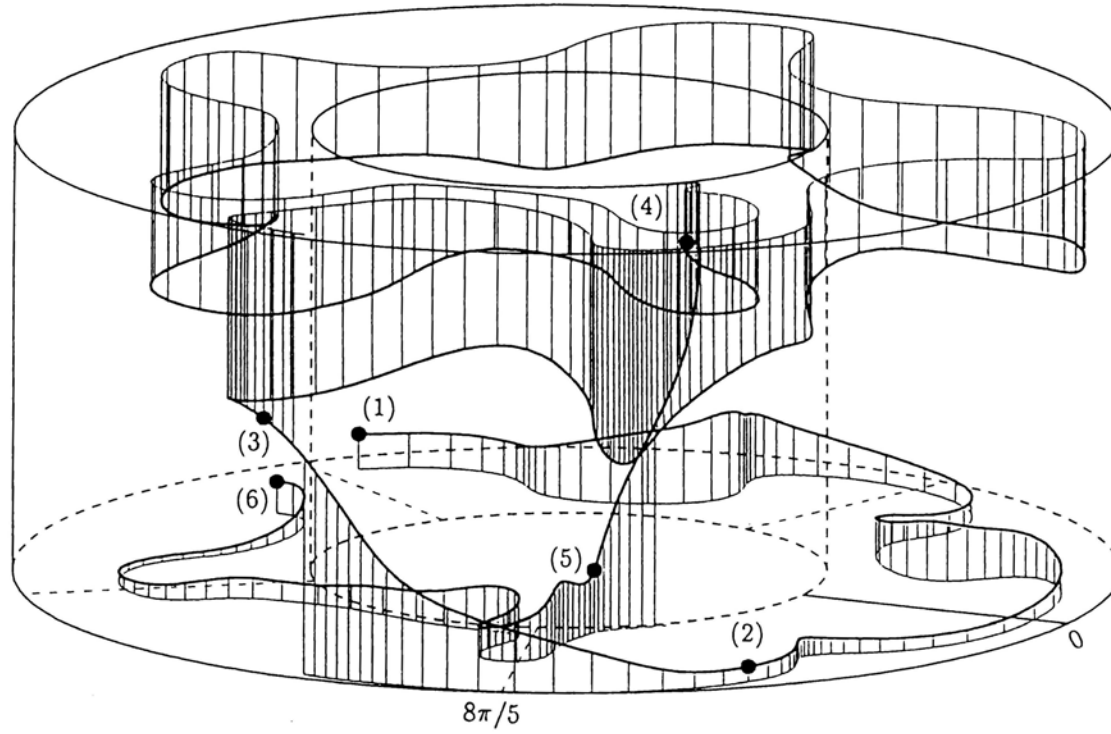
Fig. 9. Bird's-eye view of the trajectory for the upper-level jet and the lower-level jet. Labels correspond to times; t = (1) 25590s, (2) 25748s, (3) 25794s, (4) 26100s, (5) 26136s, and (6) 26260s . Each interval between the labels corresponds to; (1)–(2) the lower-level jet; (2)–(3) the outer boundary layer; (3)–(4) the upper-level jet; (4)–(5) the inner boundary layer; (5)–(6) the lower-level jet. Vertical lines are perpendicular lines drawn from the trajectory to the upper boundary or to the lower boundary every two seconds, whose direction is changed according to whether the height of the particle exceeds the half level or not.
