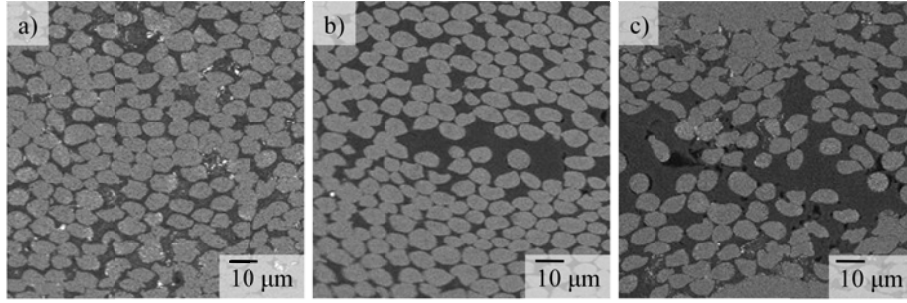
Fig. 2. Employed amount of PyC in a typical region of composite, normal to the fiber direction of a) specimen thin@I,T , b) specimen thin@I , and c) specimen thick@I for interface.
