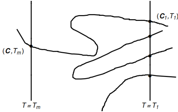
Fig. 5.15. Sketches for different possibilities for the curve c(s) . Along the curve K(C, T) \equiv 0 .
