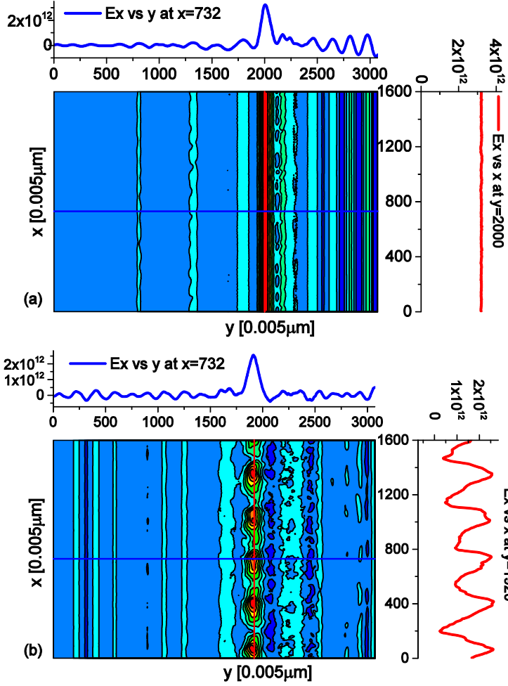
Fig. 3.13. The generation of the solitons with a = 0.5 and B_0 = 3.8kT in the 2D simulations for L_x = 8\mu\text{m} at (a) t = 139\text{fs} ; and (b) t = 157\text{fs} . The top subplot in (a) and (b) correspond to x = 732 and the right subplot in (a) and (b) correspond to y = 2000 and 1920 , respectively
