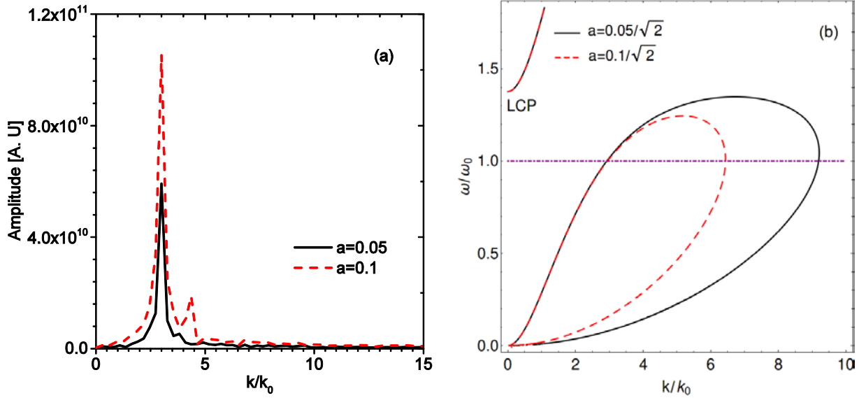
Fig. 2.5. (a) The spectrum of the wavelength for the propagation modes depicted in Fig. 2.4(a) and (b). The spectrum analysis is done between the region y = 1400 and y = 2000 (b) The enlarged plot of the dispersion relations for a = 0.05/\sqrt{2} and a = 0.1/\sqrt{2} . Notice that in the simulation the laser is linearly polarized, hence the effective intensity for the right hand circularly component should be divided by a factor of \sqrt{2} .
