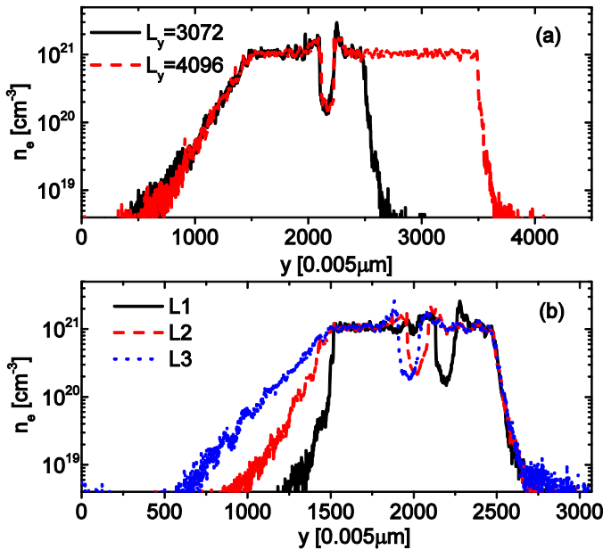
Fig. 3.11. The soliton position dependence on uniform plasma length (a) and characteristic length of the pre-plasma (b). The parameters are a = 0.5 , B_0 = 3.5kT for (a) and B_0 = 3.8kT for (b). “L1”, “L2” and “L3” in (b) represent the cases without pre-plasma, with pre-plasma of characteristic length 82 and 164, respectively.
