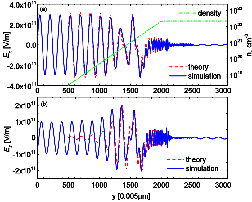
Fig. 3.6. (a) The spatial profile of E_x (left axis) and initial density profile (right axis); (b) the spatial profile of E_z . The parameters are B_0 = 18\text{kT} , a = 0.05 and n_0 = 13.3n_c .
