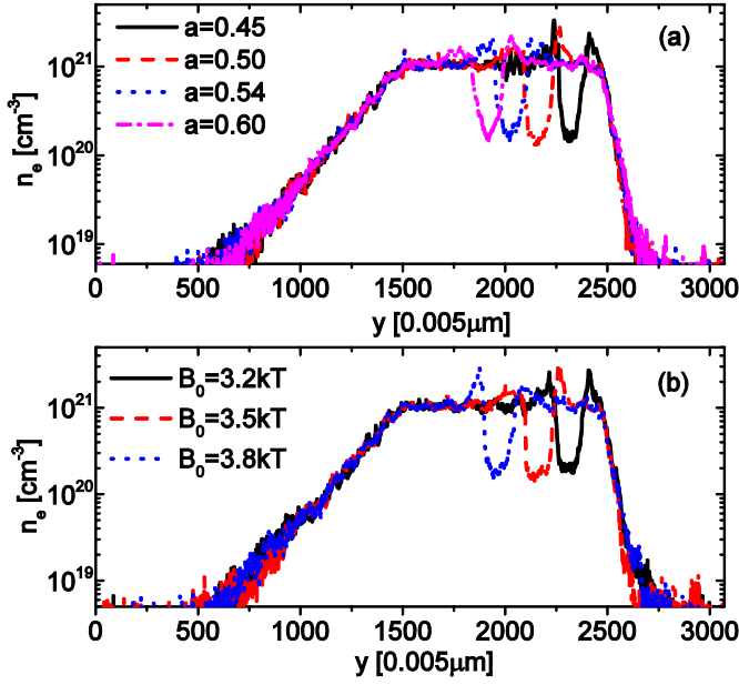
Fig. 3.10. The soliton position dependence on the laser intensity (a) and magnetic field strength (b). In (a) B_0 = 3.5kT , and in (b) a = 0.5 .
