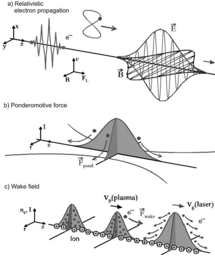
Fig. 1.3. (a) The relativistic electron motion inside the linearly polarized laser field; the Lorentz force pushes the electrons forward which results in an “8-figure” motion in the average rest frame. (b) The laser intensity versus propagation ( z ) and radial ( r ) directions; the effective Lorentz force pushed the electrons out of the high intensity areas. (c) Plasmas density versus z and r ; the ponderomotive force pushes the electrons and the charge separation between electrons and ions produces a strong longitudinal static electric field which can be used to accelerate the electrons. [Adapted from H. Schworer [8]].
