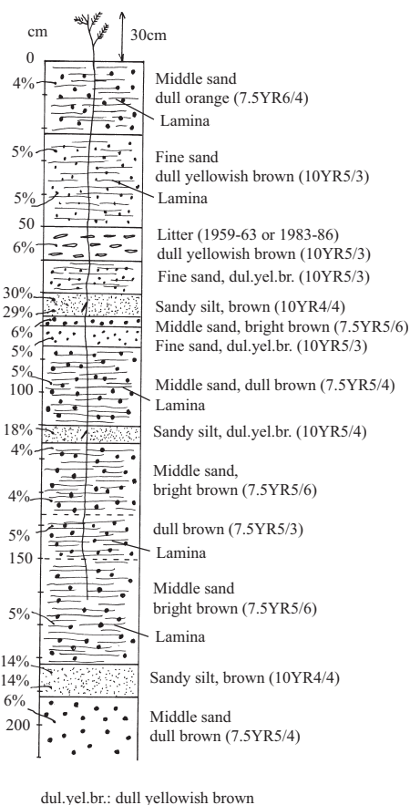
Fig. 16. Another soil profile at Quadrat S in Site 1 (Fig. 4).
