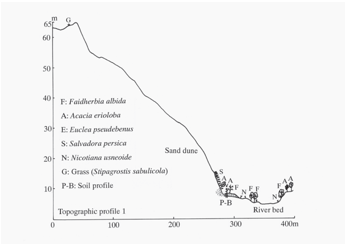
Fig. 7. Topographic profile 1 at Site 1 (Fig. 4).
