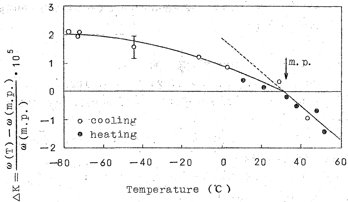
Fig. 1 Temperature dependence of Knight shift of Ga^{69} in liquid Ga .
