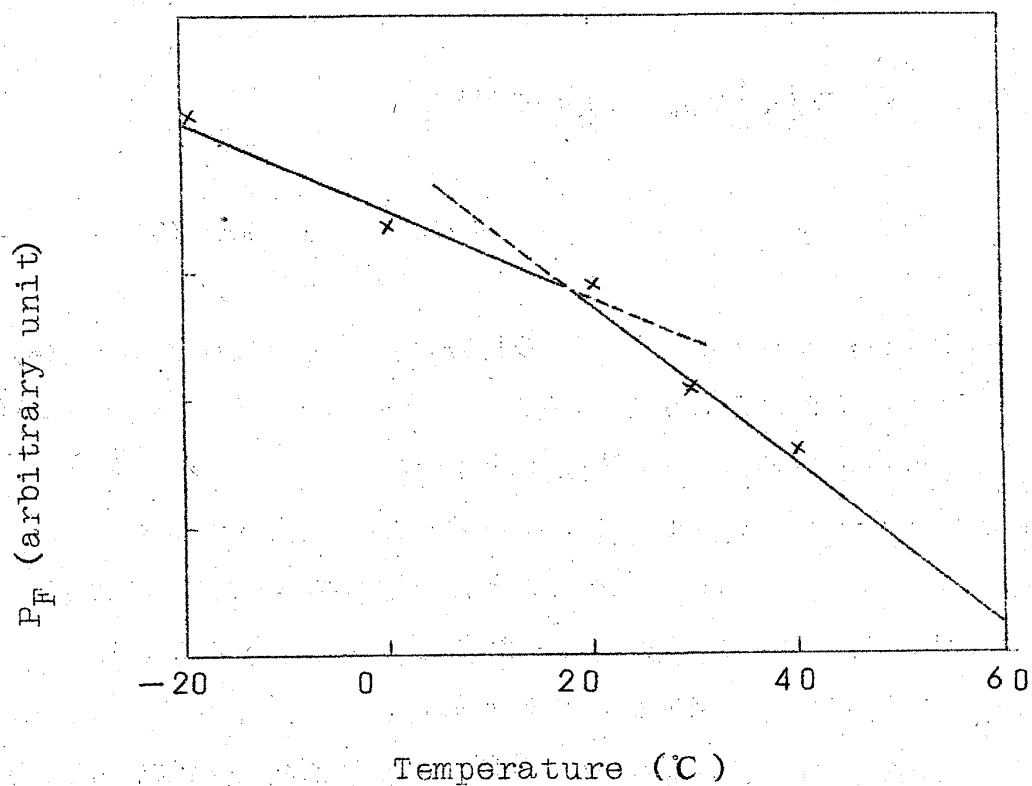
Fig. 2 Temperature dependence of P_F in liquid Ga .
