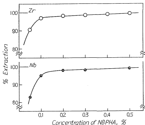
Fig. 3. Effect of NBPCHA concentration. —○— zirconium, —●— niobium.
