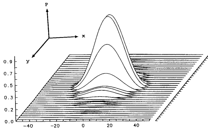
Fig. 4 Calculated field distribution from the TE_{10} mode. ( z_i = 24\lambda , \lambda = 3.0 mm, a = 5.0 mm, b = 2a )
