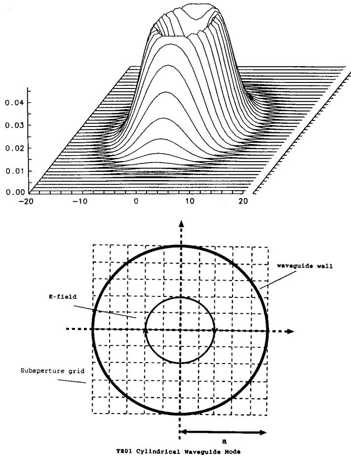
Fig. 5(a) Calculated field distribution from the TE_{01}^o mode. ( z_i = 6\lambda , \lambda = 3.0 mm, a = 5.0 mm)
