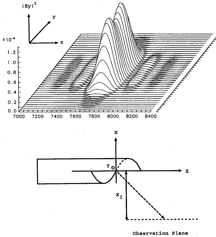
Fig. 7 Calculated field distribution from the TE'_{15,2} mode (Far-field, x_i = 9.5 m, f = 140 GHz, a = 12.8 mm).
