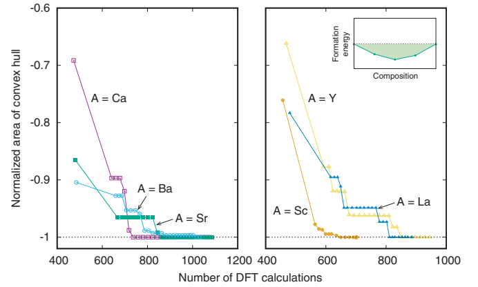
FIG. 4. Convergence behavior of the convex hull of formation energy in Bayesian optimization for \text{ACuO}_{3-x} systems. The vertical axis indicates the area of the convex hull below the line indicating zero formation energy, schematically illustrated as the shaded area at the top of the right panel. The area is normalized by the area of the converged convex hull.
