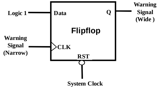
Fig. 8. Circuit for generating wide warning signal from narrow warning signal
