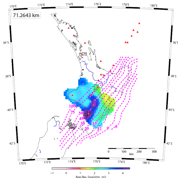
Fig. 3 3-D style plots at three depths of 1-D resistivity structure models for 28 sites calculated using the rotational invariant of the MT response function; SSQ impedance (e.g., Rung-Arunwan et al., 2016). Red triangles represent active volcanoes. Pink broken lines represent isodepth contours of the upper surface of the subducting Pacific Plate (Williams et al., 2013).
