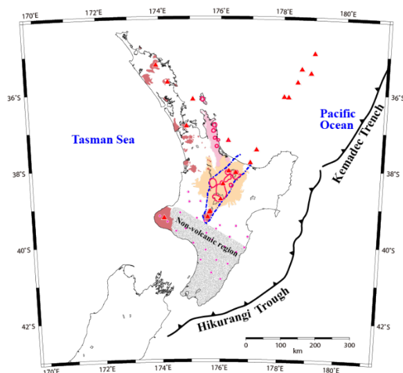
Fig. 1 Location of long-period MT sites, shown in pink dots, and representative geographic features in the North Island. Red triangles and magenta outlines indicate active Quaternary volcanoes and caldera rims, respectively. Orange area shows the distribution of pyroclastic flow deposits of ignimbrite and rhyolite, and brown area shows pyroclastic flow deposits of basalt and andesite. Blue broken line represents the edges of the Taupo volcanic zone (e.g., Briggs et al., 2005; Williams et al., 2013). Grey area represents a non-volcanic region.
