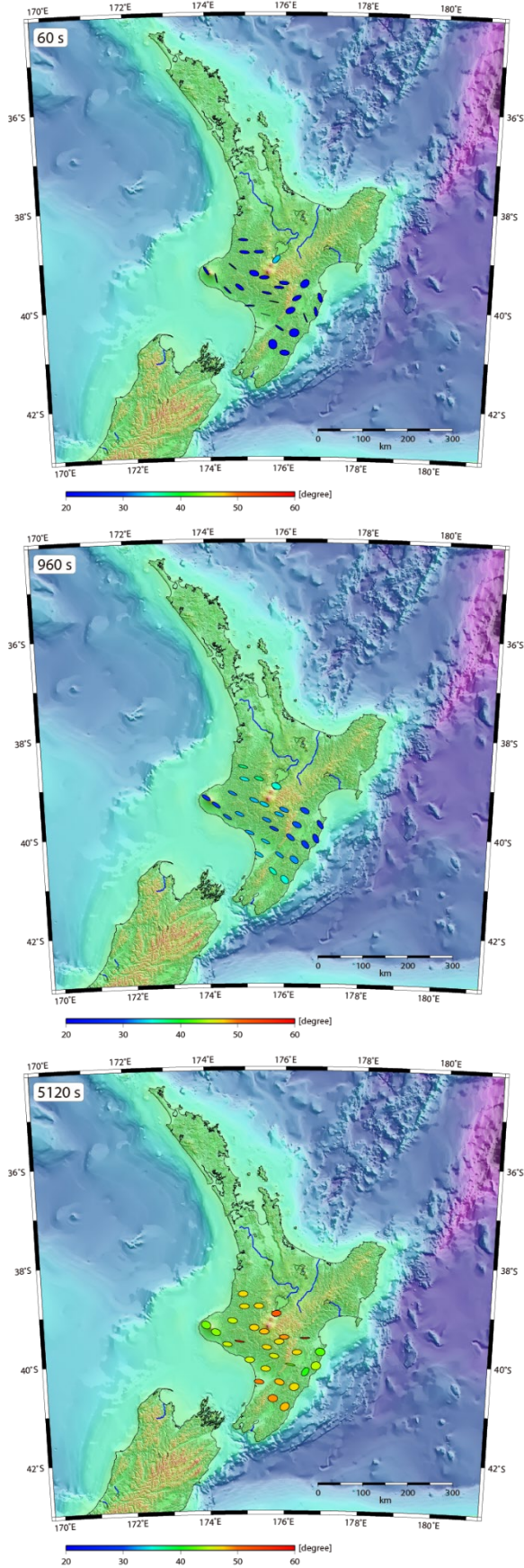
Fig. 2 Phase tensor derived from three periods (60, 960, and 5120 seconds) of the MT
