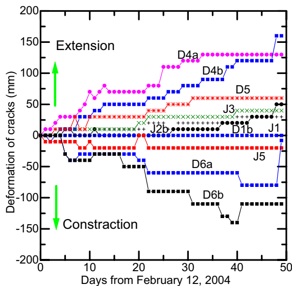
Figure 6 Measured results of crack deformation in Block-I
