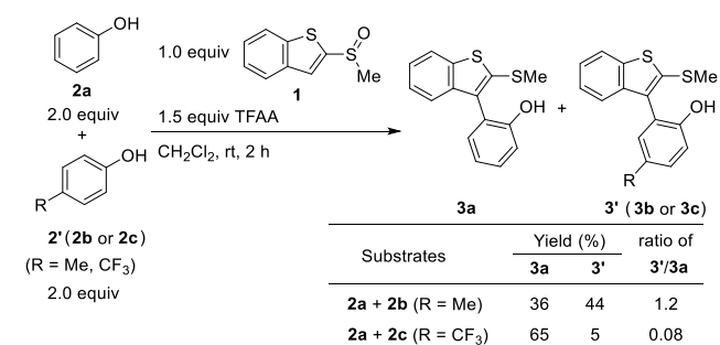
Scheme 2. Substituent effects on the phenols; yields were determined by ^1\text{H} NMR spectroscopy.
