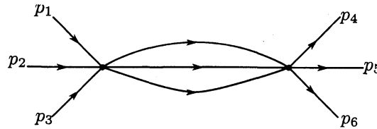
Figure 3. The Feynman graph G_0 .
