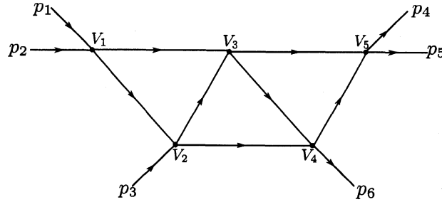
Figure 8. The truss-bridge graph T_3 .
