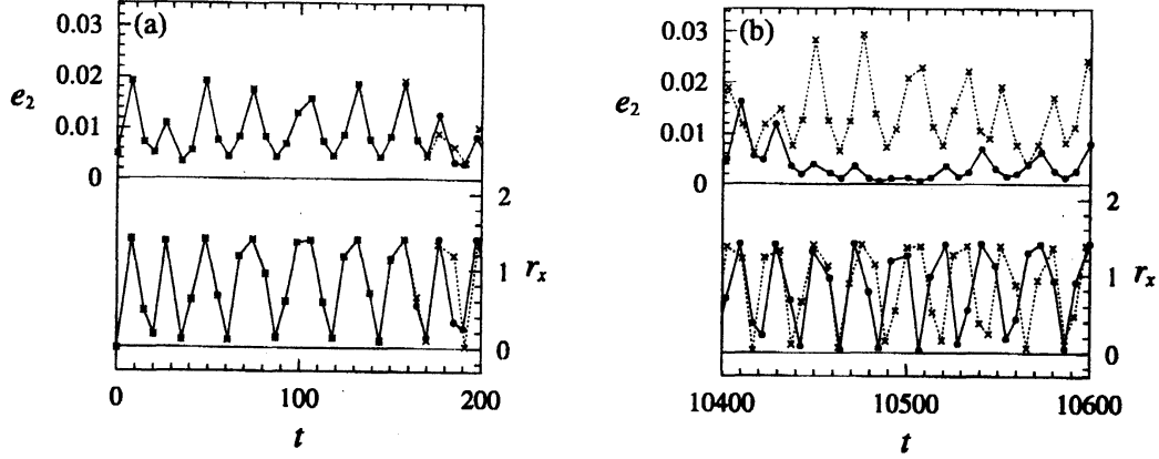
Fig. 6. The second mode energy e_2 of the y -component and the distance r_x from the invariant manifold \mathcal{M} (the y -hyperplane) for two trajectories with slightly different initial conditions for \beta_1 = 0.5 , \beta_2 = 1.5 and H = 0.01 : (a) small t ; (b) large t .
