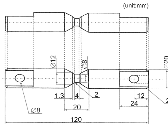
Fig. 2.1 Schematic illustrations of the dimension and shape of torsion specimen
