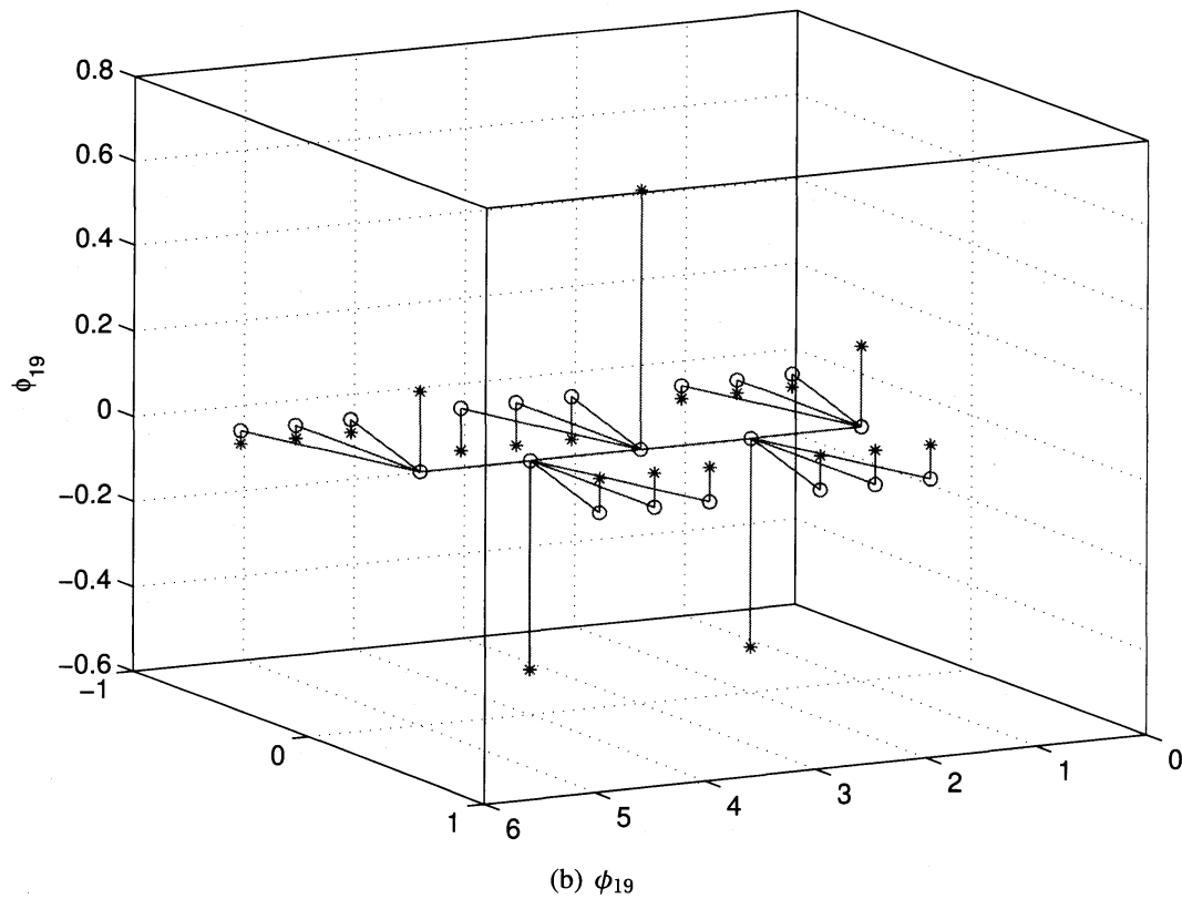
Figure 10: (a) The eigenfunction \phi_{15} corresponding to \lambda_{15} = 4 of the tree 5K_{1,3} in the 3D perspective view. (b) The eigenfunction \phi_{19} corresponding to the maximum eigenvalue \lambda_{19} = 7.1091 , which shows a bit more concentration around the central vertex.
