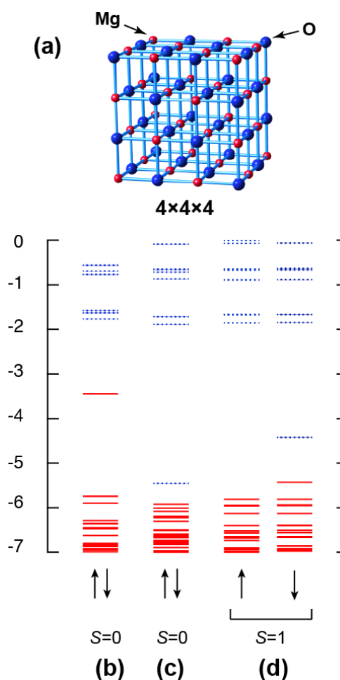
Figure 1. (a) A (4 \times 4 \times 4) -atom block of the \text{Mg}_{32}\text{O}_{32} cluster. A corner Mg (or O) atom, indicated by an arrow, is removed to create an Mg-(or O-) deficient cluster. Molecular orbital energy-level diagrams of occupied molecular orbitals (solid lines) and unoccupied molecular orbitals (dotted lines) calculated for (b) the O-deficient \text{Mg}_{32}\text{O}_{31} cluster in the spin-singlet state, (c) the Mg-deficient \text{Mg}_{31}\text{O}_{32} cluster in the spin-singlet state, (d) the Mg-deficient \text{Mg}_{31}\text{O}_{32} cluster in the spin-triplet state.
