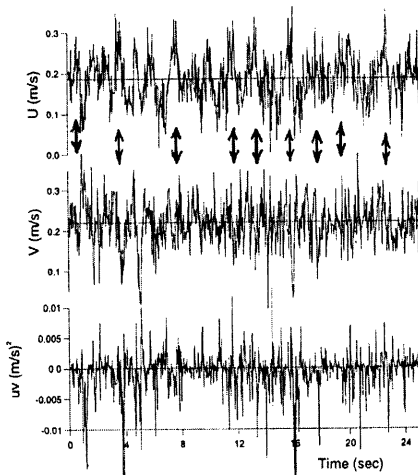
Fig. 7 Temporal variation of velocity U and V at a point within the interfacial boundary
