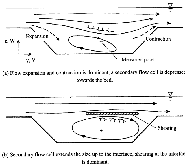
Fig. 4 Secondary flow fluctuation and interaction processes
