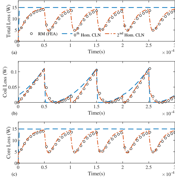
Fig. 6. EC losses on entire domain (a), coil (b) and core (c)
