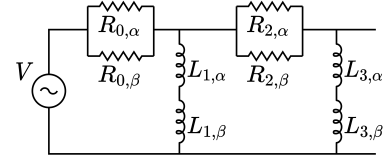
Fig. 8. CLN with divided parameters.
