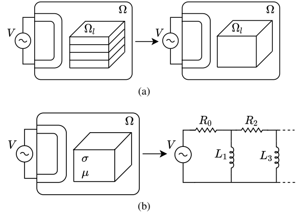
Fig. 1. (a) homogenization method as a material-scale MOR and (b) CLN method as a machine-scale MOR.
