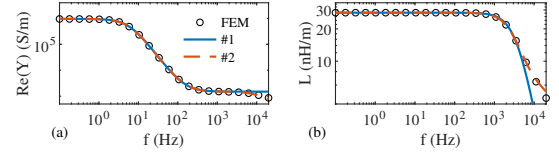
Fig. 4. Frequency responses obtained with RM, 2^{nd} order Homogenization and its equivalent CLN (#1: single stage CLN, #2: two stage CLN).
