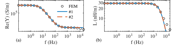
Fig. 3. Frequency responses obtained with RM, 0^{th} order Homogenization and its equivalent CLN (#1: single stage CLN, #2: two stage CLN).
