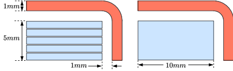
Fig. 2. One quarter of FE model -left: RM -right: homogenized.
