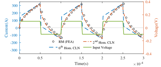
Fig. 5. Transient response to rectangular excitation.
