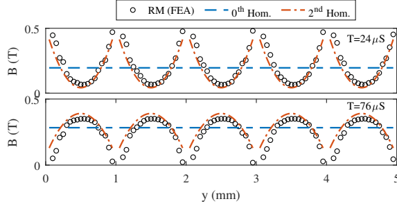
Fig. 7. The distribution of magnetic field at the center-line.
