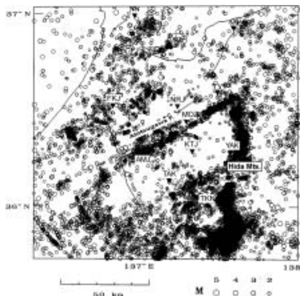
Fig.1. Epicenter distribution of earthquakes in the north-western Chubu district, central Japan from 1985-2002 determined by the Kamitakara Observatory, Kyoto University. Major active faults are shown by solid lines.
