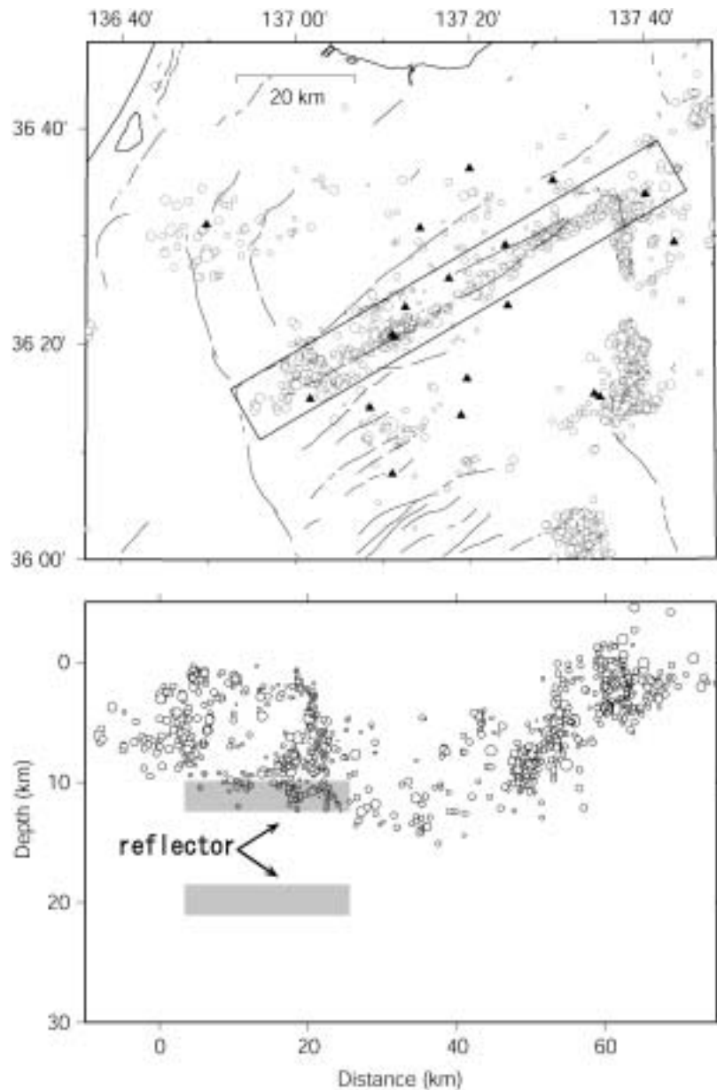
Fig10 Epicenters (upper figure) and focal depths (lower figure) along the Atotsugawa fault system. Hypocenters are the same as in Figs. 3,4. Locations of the section is shown in upper figure. Triangles show stations. Reflectors obtained in this study are shown by shaded strips.
