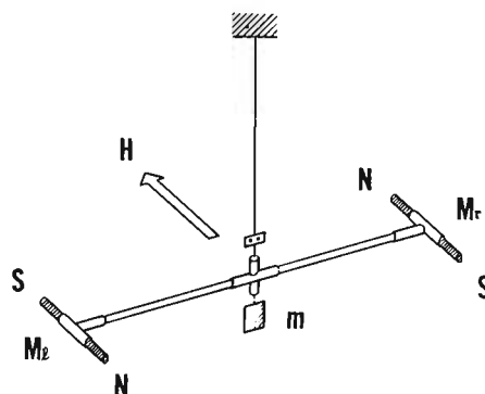
Fig. 1b. Principle of magnetic torsion balance.
