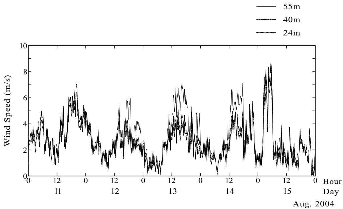
Fig. 6 Diurnal variations of wind speed on 11-15 Aug. 2004
