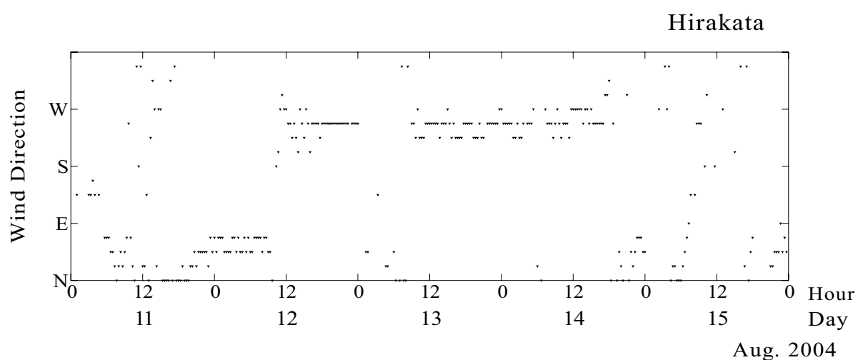
Fig. 9 Diurnal variations of wind direction at the Kyoto, Kyotanabe and Hirakata Stations of Automated Meteorological Data Acquisition System (AMeDAS) on 11-15 Aug. 2004
