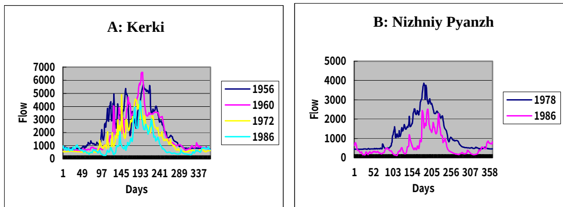
Fig. 7.1 Daily Flow Rate at Kerki (A) and Nizhniy-Pyandzh (B) from 1956 to 1986 (Tsuneo Tsukatani, et al. 2001. Unit of flow rate is \times 10^5 \text{ m}^3/\text{day} )
