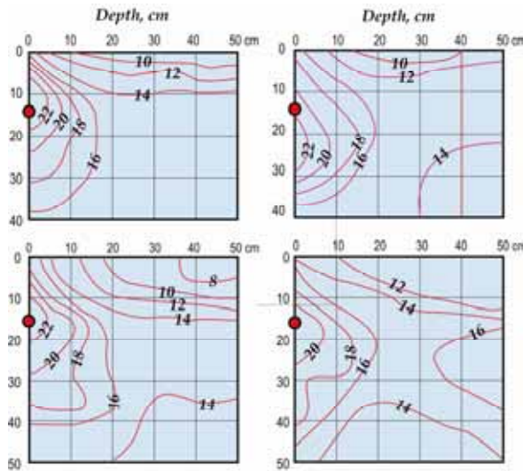
Fig. 8.7 Forming of moistening outlines during watering norm of 50 \text{ m}^3/\text{ha} , the distance between the drippers is 0.9 \text{ m} and average specific expenditure 0.007 \text{ l/s.m.}
