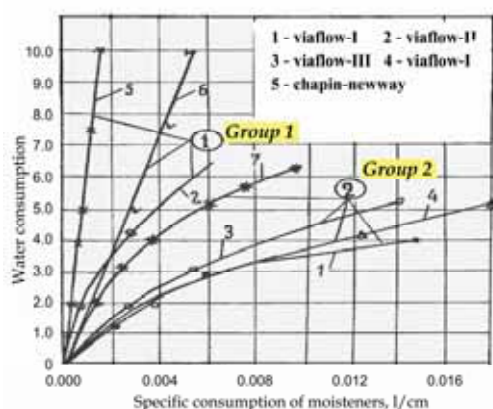
Fig. 8.2 Water consumption characteristics of drippers of various constructions
