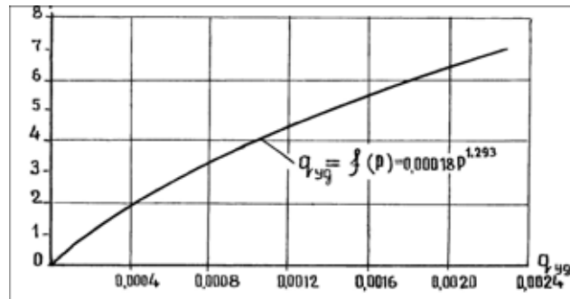
Fig. 8.9. Dependency of change of specific expenditure of drippers from the pressure of water at the depth of 0.15 m.
