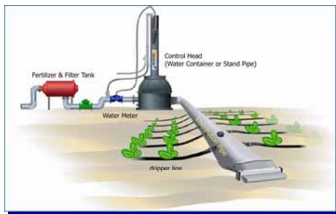
Fig. 8.1 Low Pressure System components of Netafim™ The economic new solution for flood and furrow irrigation of field crops
