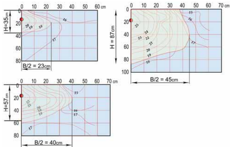
Fig. 8.7 Forming of the outline of soil moistening for various specific watering norms
