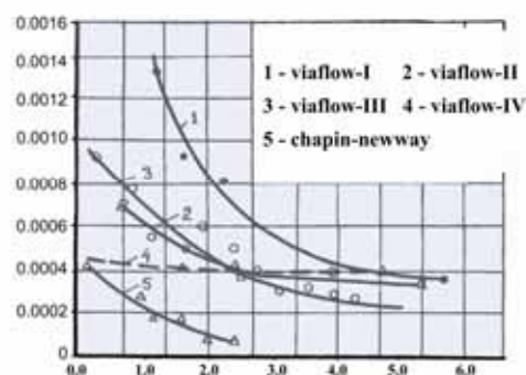
Fig. 8.3 The change in water expenditures of Viaflow and Chapin drippers depending on the irrigational norm
