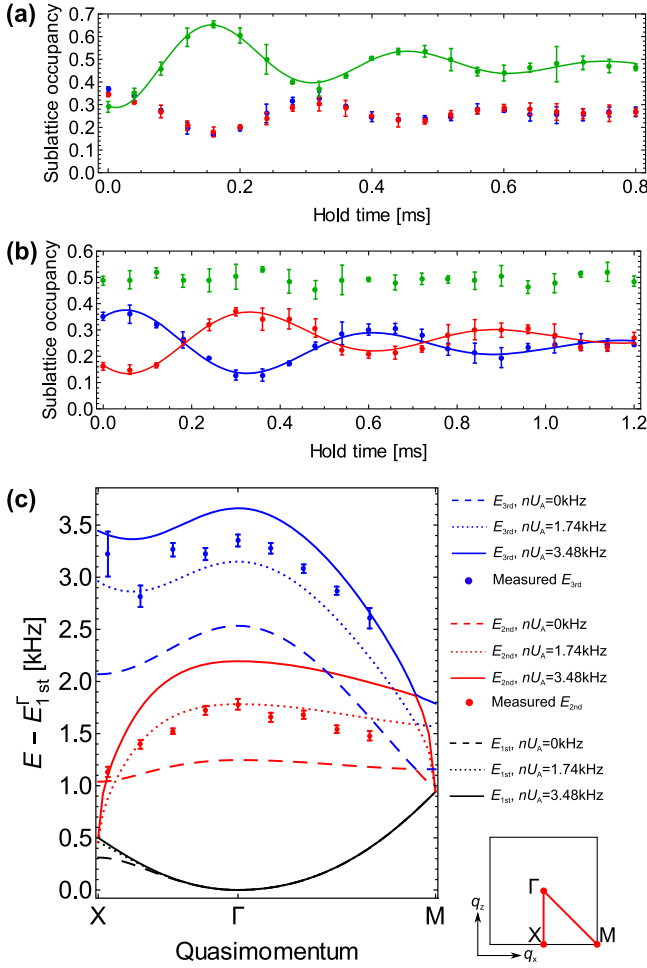
FIG. 3. (a),(b) Oscillation of the sublattice population at the \Gamma point according to (a) E_{3-1} and (b) E_{2-1} , respectively. First, we load a BEC into an optical lattice the configuration of which is different from that of a Lieb lattice. In this way, we create a superposition of (a) the 1st and 3rd or (b) the 1st and 2nd band eigenstates of the Lieb lattice. Next, we suddenly change the lattice configuration into the Lieb lattice, and take various hold time. We observe the temporal change of the sublattice populations obtained by the projection measurement described in the text. Each sublattice occupancy is normalized by the summation over all of the sublattice occupancy. Green, blue, and red circles show the A-, B-, and C-sublattice population, respectively. The error bar shows the standard deviation of three independent scans. Solid lines are fits to the data with damped sine functions(4). (c) The lowest three bands in the optical Lieb lattice of (s_{\text{long}}, s_{\text{short}}, s_{\text{diag}}) = (13, 13, 15.5) . Red and blue circles are the reconstructed 2nd and 3rd band energies, respectively. Error bars mean the fitting errors. Dashed lines are the predictions based on a single-particle theory. The dotted and solid lines are the calculations including the interaction based on the BdGE with the half and maximum densities, respectively.
