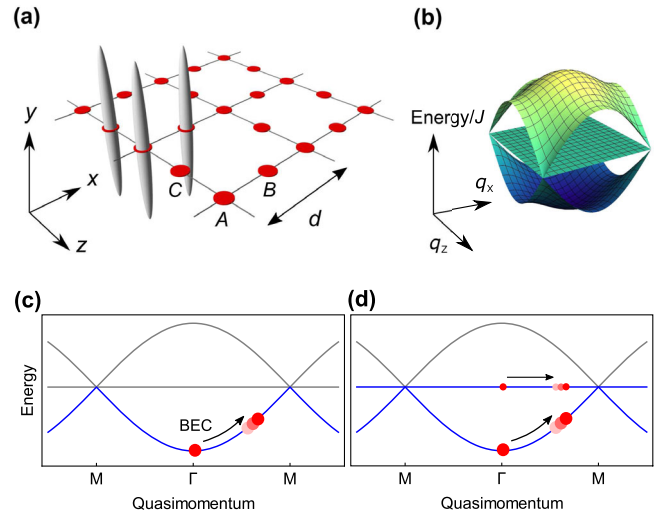
FIG. 1. (a) Schematic of Lieb lattice. In our system, the atoms are weakly trapped along the y direction, and distribute like tubes as shown in gray in the figure. (b) Band structure of Lieb lattice in a single-particle description. (c) Method for measuring dispersion of the lowest band. Red circles indicate the atomic cloud. After transporting a BEC to a desired quasimomentum, we measure the group velocity and integrate the results. (d) Method for measuring a band gap in a momentum-resolved manner. We prepare the superposition of band eigenstates, transport the atoms to a desired quasimomentum, and measure an oscillation frequency of the sublattice population.
