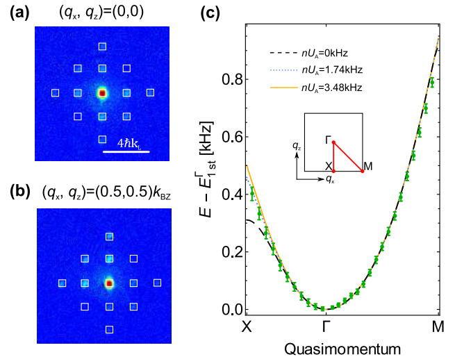
FIG. 2. (a),(b) Absorption images at quasimomentum (q_x, q_z) = (0,0) and (0.5, 0.5)k_{\text{BZ}} , respectively, where k_{\text{BZ}} corresponds to the quasimomentum at the BZ edge. The images are taken after a TOF of 14 ms. We restrict the integration region within the white squares in which the atoms are mostly detected. (c) Dispersion of the 1st band of optical Lieb lattice (s_{\text{long}}, s_{\text{short}}, s_{\text{diag}}) = (13, 13, 15.5) . The experimental data are denoted as green circles. The inset shows the first BZ. The dashed black line shows single-particle theory. The dotted blue line is the calculation for half of the maximum number density. The solid yellow line is for the maximum number density. The vertical axis shows the energy difference from the 1st band energy at \Gamma for each interaction strength. The error bar indicates the standard deviation of three independent scans.
