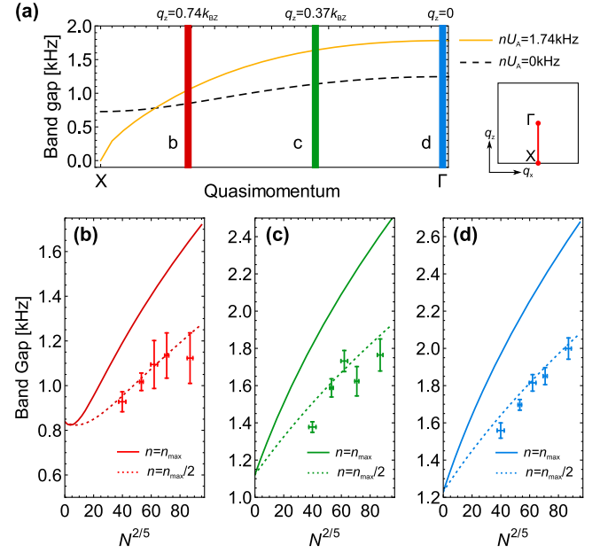
FIG. 4. (a) Band gaps from the lowest band to the 2nd band. Dashed black line is the prediction on the single particle theory of the Lieb lattice potential (s_{\text{long}}, s_{\text{short}}, s_{\text{diag}}) = (13, 13, 15.5) . Solid yellow line is the calculation including the interaction based on the BdGE. Thick red, green, and blue lines, respectively, show the quasimomenta q_z = 0.74k_{BZ} , 0.37k_{BZ} , and 0 at which we have investigated the density dependence of the band gaps. (b),(c),(d) Band gap versus the atom number for q_z = 0.74k_{BZ} , 0.37k_{BZ} , 0 , respectively. Solid and dotted lines show the calculations including the interaction based on the BdGE for the maximum and half densities, respectively. Error bars indicate the fitting errors.
