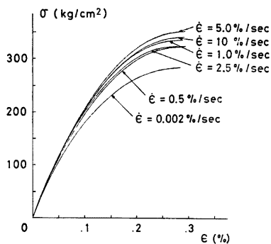
Fig. 7 Average Curves
