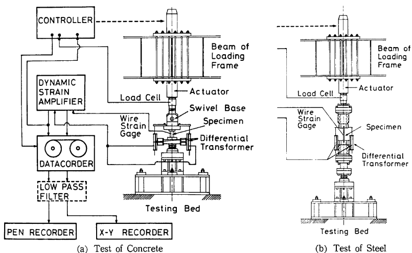
Fig. 2 Test System
