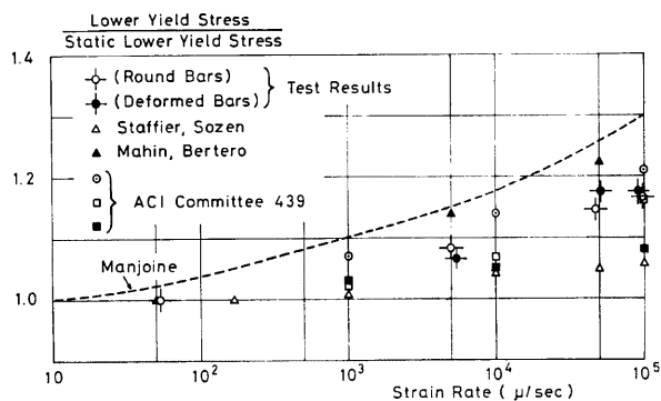
(c) Lower Yield Stress of Steel
