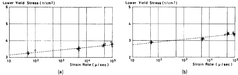
Fig. 18 Lower Yield Stress versus Strain Rate Diagram
