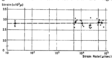
Fig. 12 Strain at Maximum Stress versus Strain Rate Diagram
