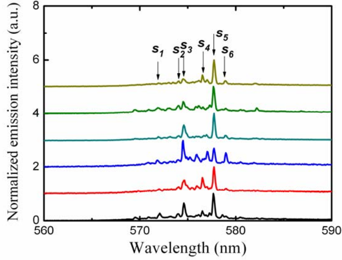
Fig. 4.6: Six of single-shot emission spectra collected at the same position on the sample; the lasing modes trend to populate in frequencies denoted by S_n ( n : 1~6). The stripe length under irradiation is 2.4 mm. The pumping pulse energy is about 2.13 \mu\text{J} .
