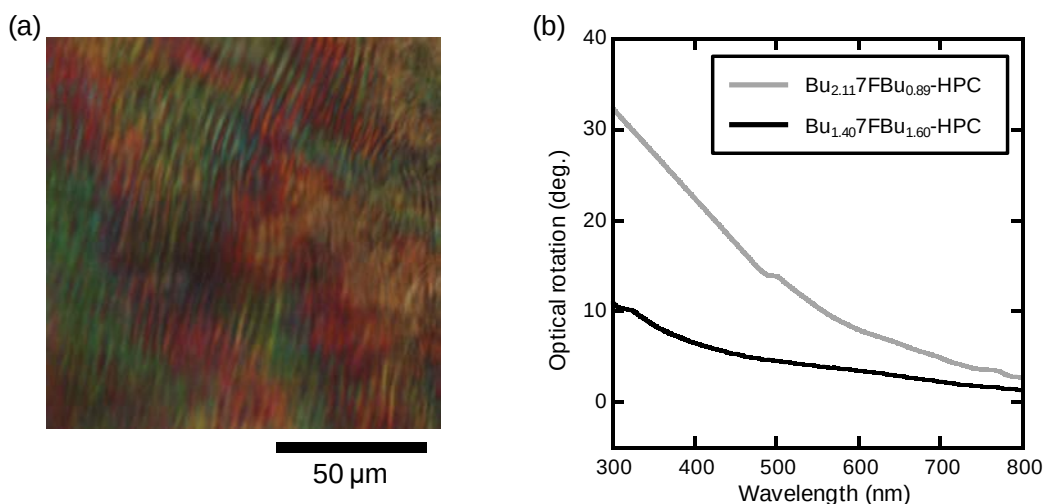
Fig. 5 (a) POM image of \text{Bu}_{2.11}\text{7FBu}_{0.89}\text{-HPC} and (b) ORD spectra of \text{Bu}_{2.11}\text{7FBu}_{0.89}\text{-HPC} and \text{Bu}_{1.40}\text{7FBu}_{1.60}\text{-HPC} . All the data were obtained at 70 °C
