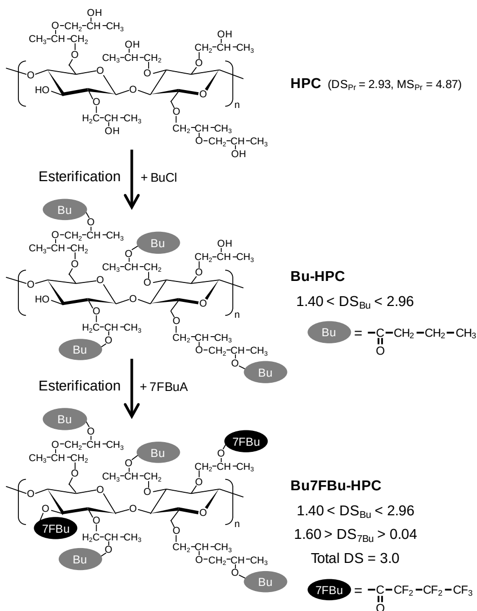
Scheme 1 Synthetic pathway to Bu7FBu-HPC from HPC
