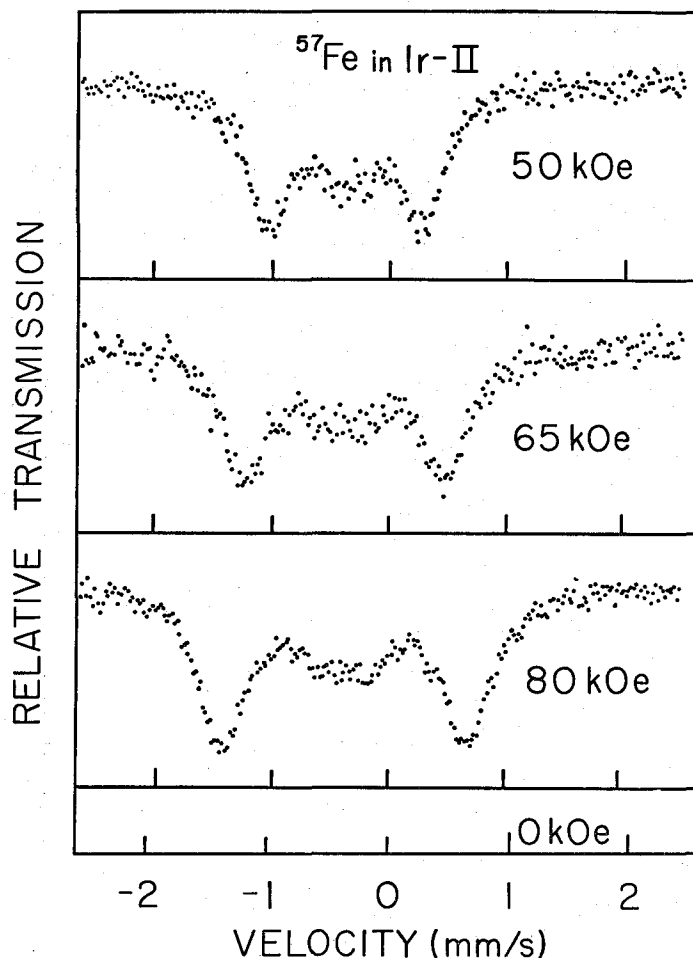
Fig. 2. Mössbauer spectra of \text{Fe}^{57} impurities in Ir-II at 4.2 K in various external magnetic fields. The direction of \gamma rays is parallel to the external field. The velocity calibration was made in the presence of external field (See Fig. 1).
