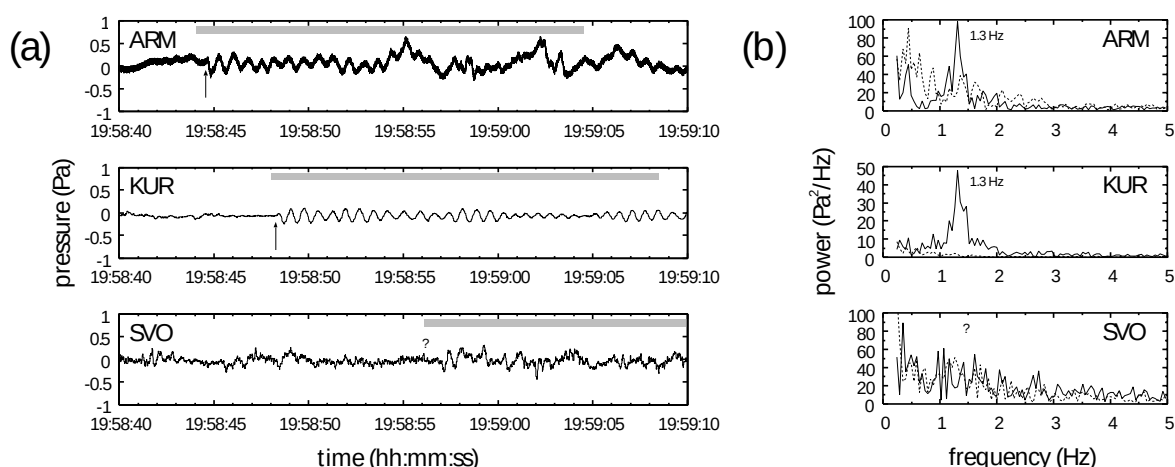
Fig. 8 (a) Monotonic infrasound waveforms observed on June 15 (Yokoo et al., 2008). It is difficult to recognize these signals at SVO. (b) FFT power spectrum for the gray colored periods in (a), 20.48 s. Dashed lines are those of the background at the periods of 1 min before the arrivals.
