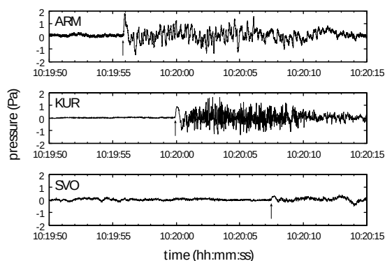
Fig. 6 Infrasound waveforms associated with the eruption on May 24. Arrows indicate the arrival time of the waves at each station.
