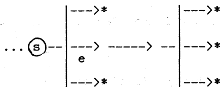
fig. 4 Failed node
