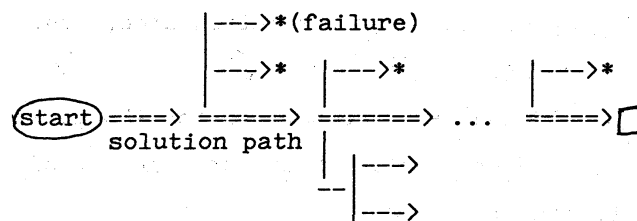
fig. 3 Solution path
