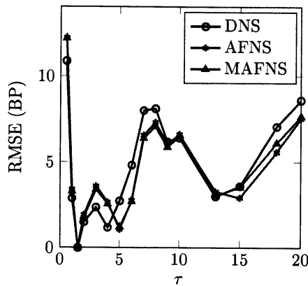
Figure 8: RMSE (JGB)
