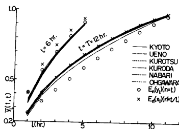
Fig. 6. Comparison of y_l(1, t) by the observation points for t=6(\text{hr.}) and t=T=12(\text{hr.}) . y_l(1, t) represents the maximum distribution rate to l hours in the maximum t -hour-rainfall of 12-hour-rainfall of which recording unit is 1 hour, and bar means the average value.
