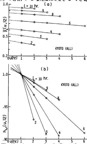
Fig. 10. An example of effects of recording unit u (hr.) on the values y_l which can be estimated. (a) Relation between y_l(u, T) and u . (b) Relation between h_{l,1}(u, T) (Eq.(10)) and u .
