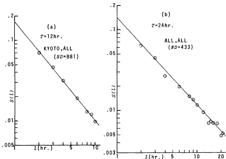
Fig. 11. Examples of relation between l (hr.) and S(l) . Where, S(l) is the absolute value of inclination of straight line which is fitted to the relation between h_{i,1}(u, T) and u . (a) is the case of Fig. 10, and (b) is the case of T=24 (hr.) shown in Table 1.
