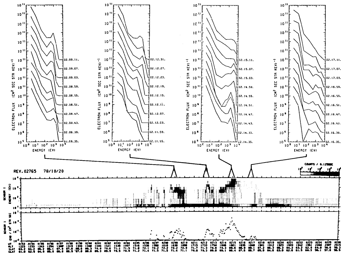
Fig. 5.8 Electron precipitation pattern in the evening hours.
