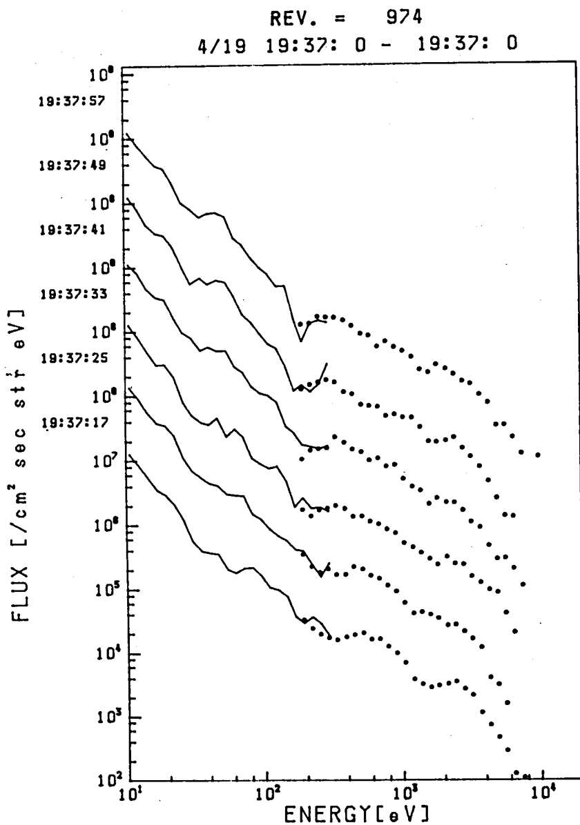
Fig. 5.41 Intercomparison between the LE and HE results.
