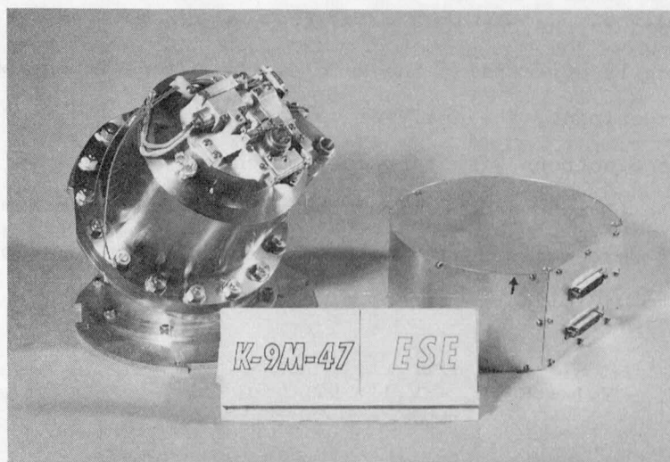
Fig. 3.10 Photograph of the sensor (left-hand) and the electronics (right-hand) of the electron spectrometer on board K-9M-47.
