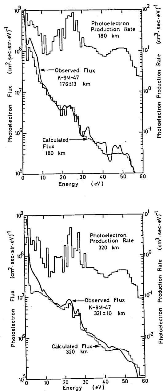
Fig. 4.17 Calculated and Measured energy spectra of the photoelectron fluxes for altitudes of 180 km (upper panel) and 320 km (lower panel). The production spectra of primary photoelectrons are also shown for comparison with the steady-state spectra.
