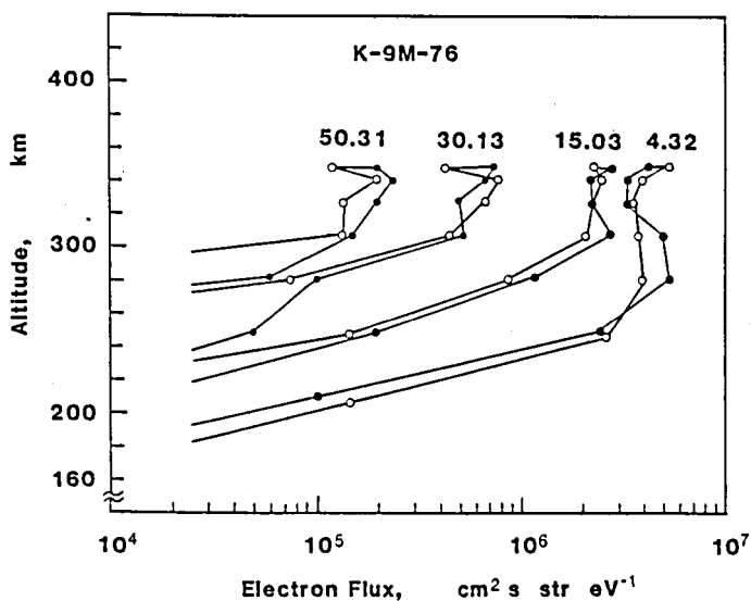
Fig. 4.24 Altitude profiles of the electron fluxes at four selected energies observed by the K-9M-76 experiment. Open and solid circles show the upleg data and the downleg data, respectively.
