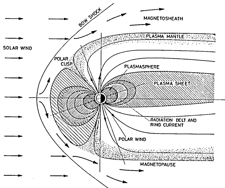
Fig. 1.2 Noon-midnight cross section of the magnetospheric plasma domains. (after H. Rosenbauer et al., 1975)
