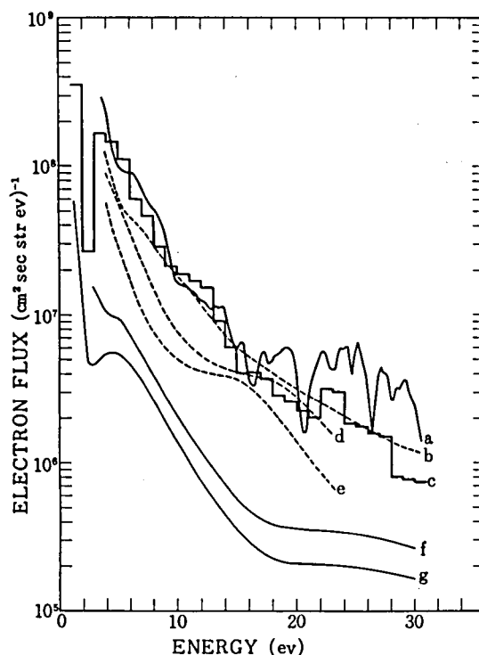
Fig. 4. 2 Comparison of the present result with other observational and theoretical spectra at the ~200-km level: a, present study; b, Knudsen et al. [1970]; c, Ogawa [1971]; d, Doering et al. [1970]; e, Doering et al. [1970]; f, Hays and Sharp [1973]; and g, Hays and Sharp [1973]. See Table 4.2 for solar zenith angles and altitude. Spectra f and g have been multiplied by the factor 1/4\pi .
