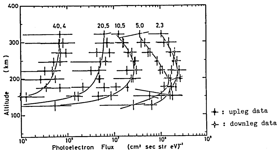
Fig. 4.14 Altitude profile of the photoelectron flux at several energies as indicated.
