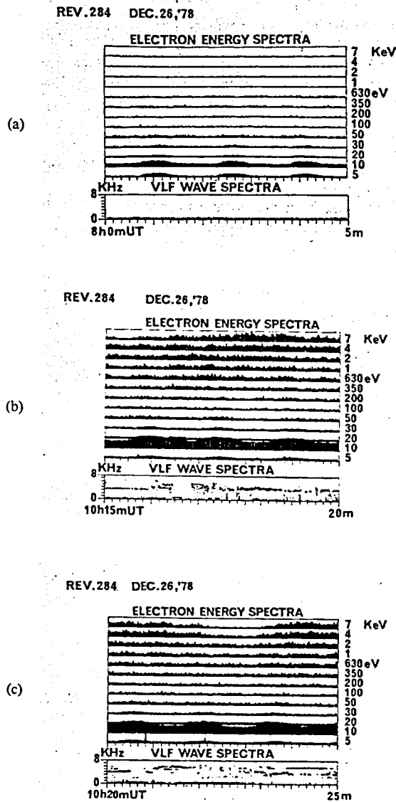
Fig. 5.30 A detailed comparison between wave dynamic spectra and electron fluxes at each channel of electron analyzer.
