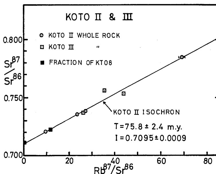
Fig. 8. Rb-Sr evolution diagram for KOTO-II and III. The isochron is drawn through data points of KOTO-II.
