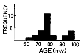
Fig. 9. Frequency of biotite ages of granitic rocks around the Lake Biwa.
