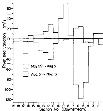
Fig. 9. Variation of river bed from May to November 1975 (Upstream of the measuring flume).
