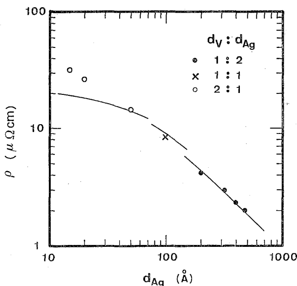
Fig. 2. Normal-state resistivity as a function of Ag-layer thickness. Solid curves are calculated on the assumption of the bulk resistivity in the V layers ( 15 \mu\Omega \text{ cm} ) and the thickness-dependent resistivity in the Ag layers.
