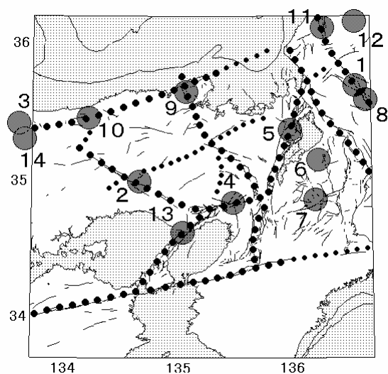
Fig. 1 Block boundary in Kinki region and historical large earthquakes ( Watanabe, 2004 )
