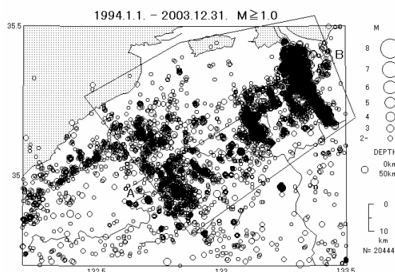
Fig. 6 Seismic activity in eastern Shimane pref. There are two active zones perpendicular to the Japan Sea coast. The east one is the aftershock area of 2000 western Tottori earthquake and the west one is Mt. Sanbe area. Time-space distribution of epicenters in the surrounded area is shown in Fig. 7 ( Watanabe, 2004 ).
