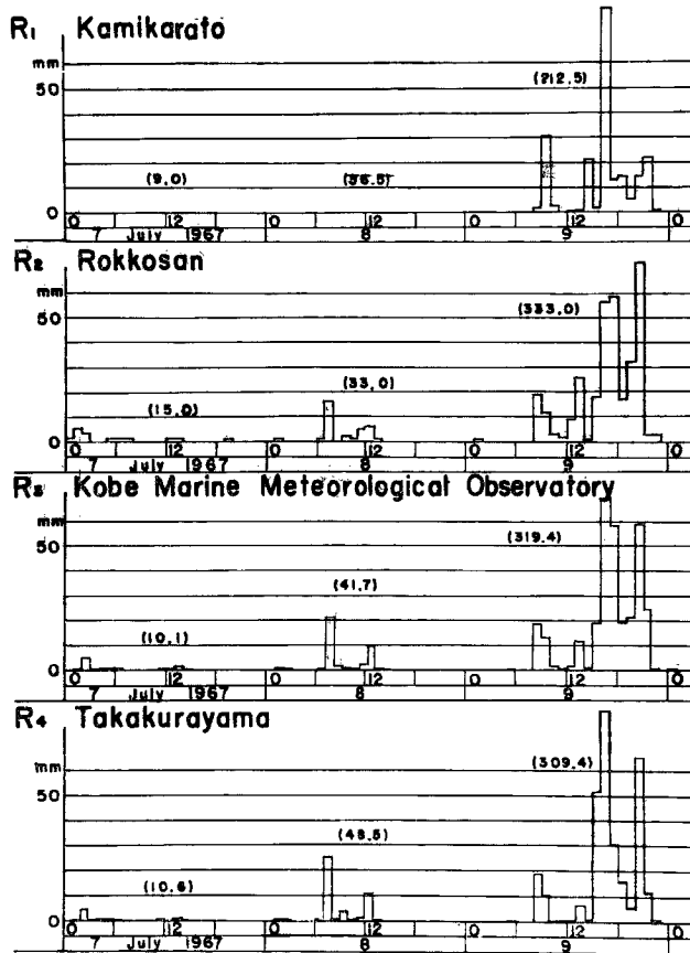
Fig. 2 Hyetographs recorded at rain gauge stations R 1 , R 2 , R 3 and R 4 in Fig. 1.
